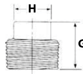
NO. 6 SQUARE PLUG
